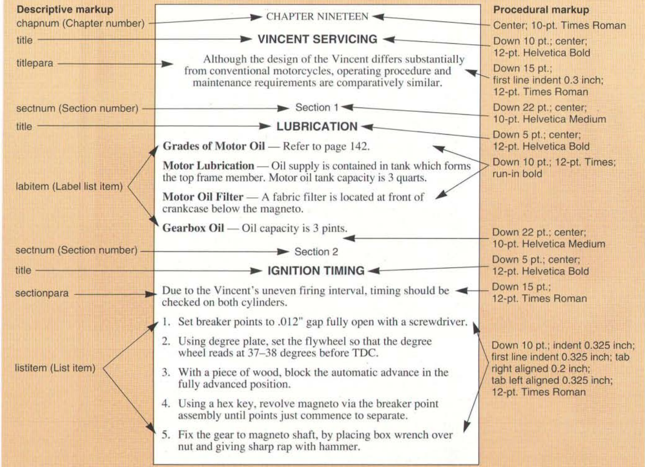
Figure 1: This page is marked up with simplified versions of both procedural and descriptive markup languages. Note the mapping between the two languages; it forms the essence of a style sheet. The text appearing on the page was taken from Modern Motorcycle Mechanics (Nicholson Brothers Motorcycles, Ltd., 1974).
